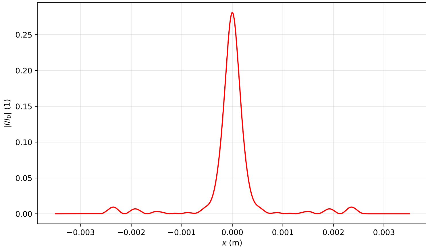
Intensity profile I(x, y = 0, z = 2.866)/I_0 , P_{in}=8.0P_{cr} , artificial time
